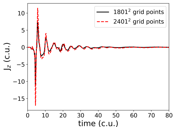
Figure 8. The J_z current density profiles at the X-point for two setups at 1 MK base temperature and anisotropic thermal conduction are overlotted. The black line corresponds to the lower-resolution setup with 1801^2 grid points, and the red dashed line to the higher resolution setup with 2401^2 grid points.
