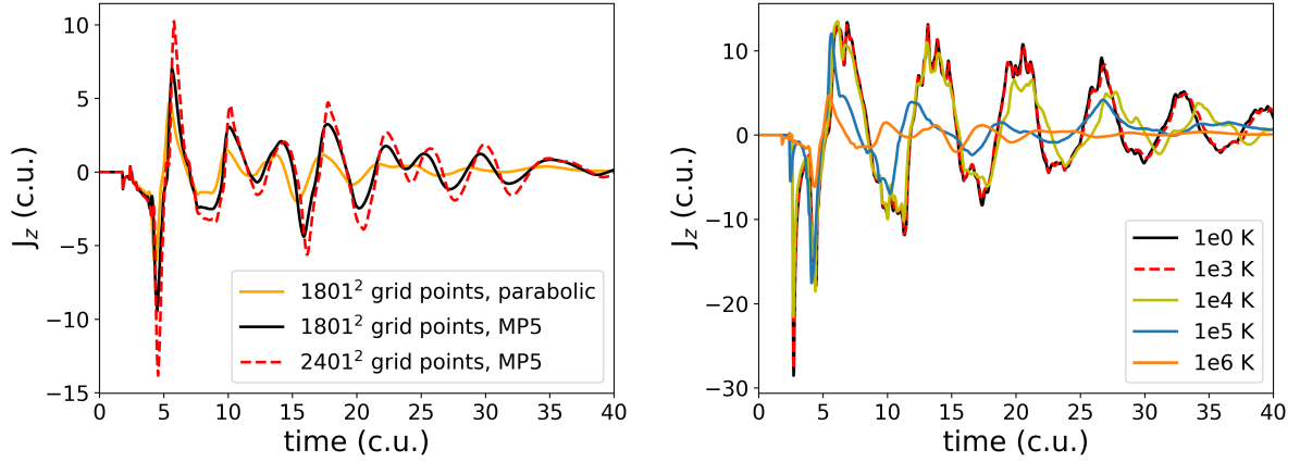
Figure 12. Left panel: a comparison plot of different setups with 1 MK base temperature without thermal conduction. Two of the profiles are for the lower-resolution setups for different spatial reconstruction methods (MP5 and Parabolic), and the third is for the high-resolution setup with the MP5 spatial reconstruction method. This plot connects the results of the temperature parameter study to the high-resolution base setup on which we focused in this study. Right panel: plot of the J_z current density profile for all the setups with the different base temperatures that were used in this parameter study. For these setups, we have not used thermal conduction.
